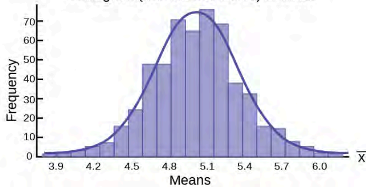
Histogram (with Normal Curve) of Mean
