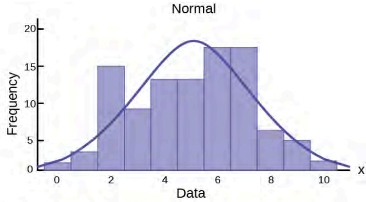
Histogram (with Normal Curve) of Mean
